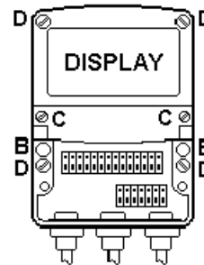
Fig 5 BA484DF-F installation procedure
